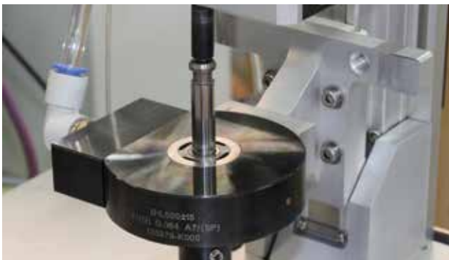
O.D. measurement
