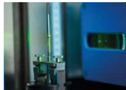
Workpiece-specific clamping devices for measuring small and very small parts
